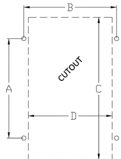
Mounting Dimensions
