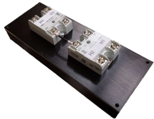
SCR Power Controller Assembly (mounted through panel wall, 3 Phase version shown)
