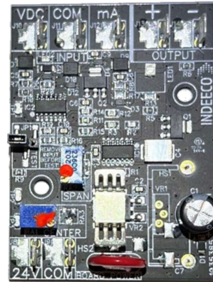
Drives up to 4 controllers per Input Board with Pulsed 24VDC, 1 Second time base
