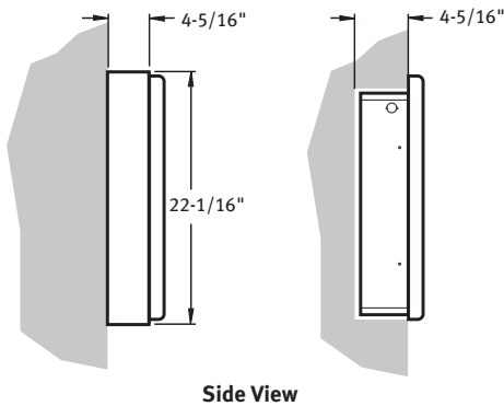
Required Wall Depth Opening
