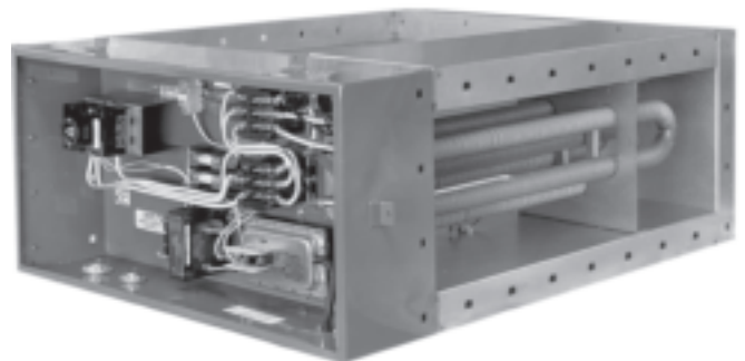
Marine Duct Heater with Side Mount Terminal Box
